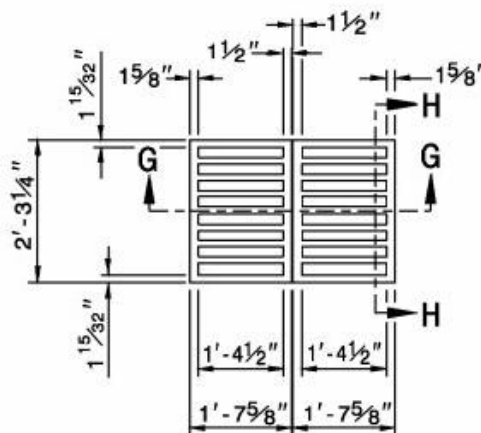
PLAN OF GRATING CAST IRON
