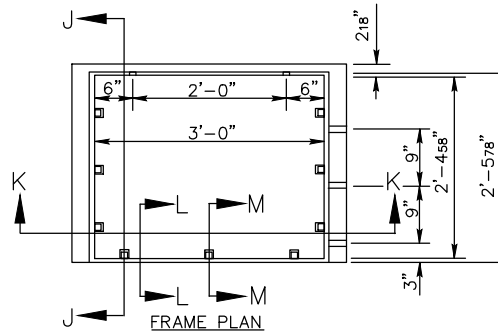
FRAME PLAN
