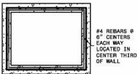
PRECAST RISER PLAN
