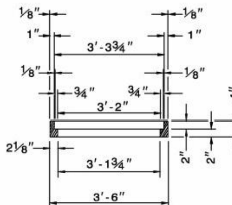
SECTION E-E
