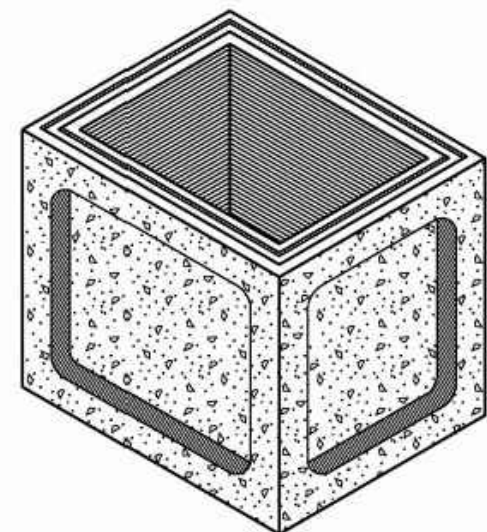
WAFFLE WALL ISOMETRIC VIEW
