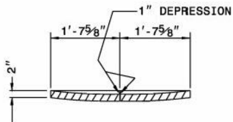
SECTION G-G
