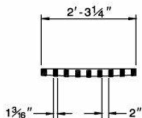
SECTION H-H
