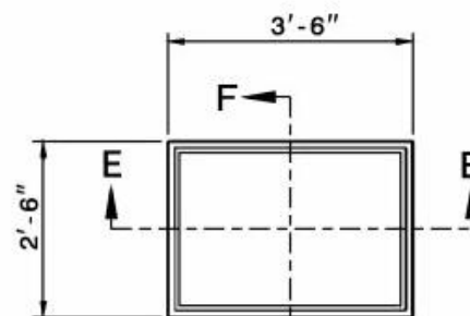
PLAN OF FRAME CAST IRON
