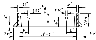
SECTION - KK
