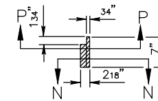
SECTION - MM
