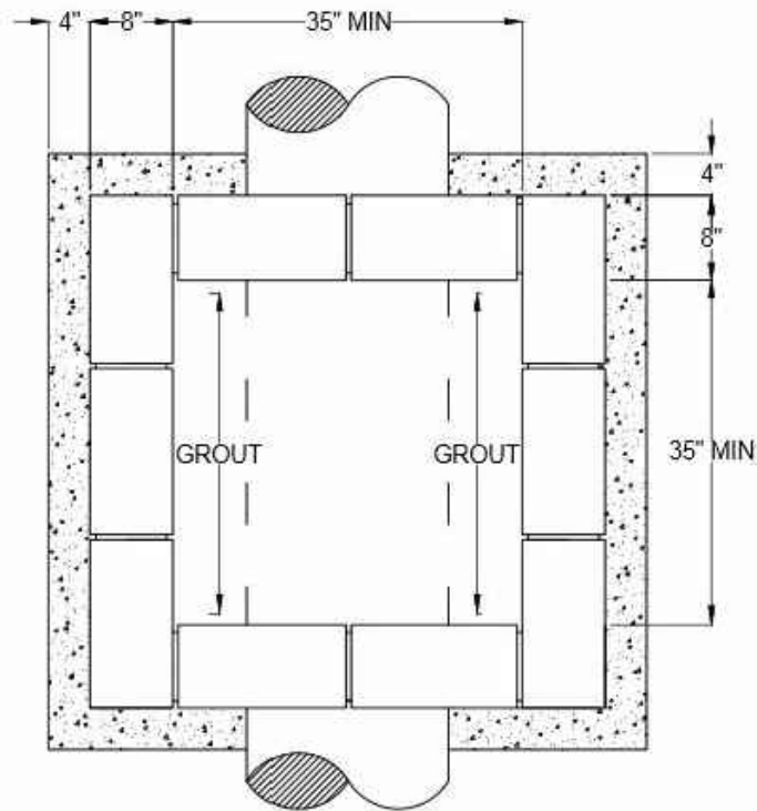
PLAN
