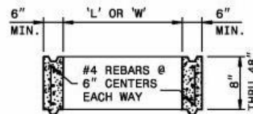
TYPICAL PRECAST RISER SECTION
