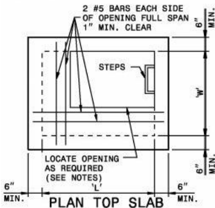
PLAN TOP SLAB
