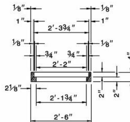
SECTION F-F
