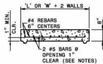
TYPICAL SECTION TOP SLAB
