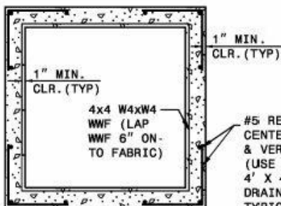
PLAN VIEW OF BASE UNIT
