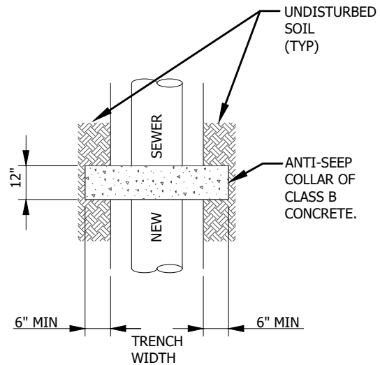
PLAN
