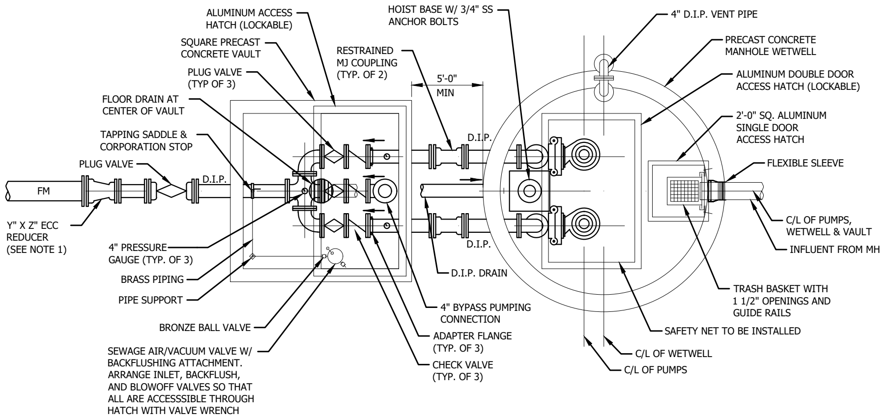
PLAN
